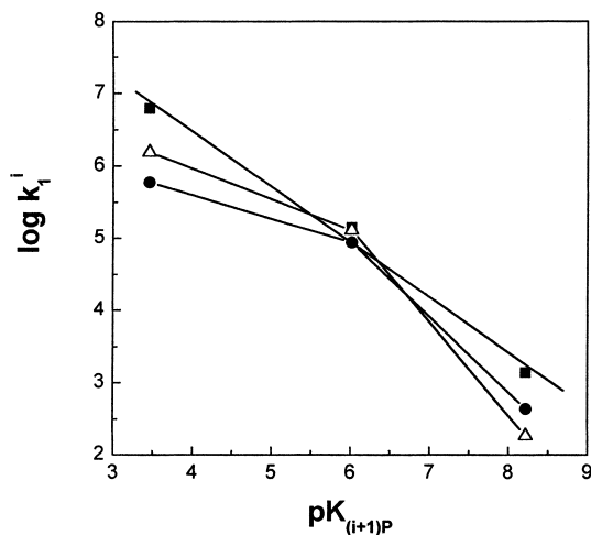
Fig. 5. Brønsted plot for the PLP-TRP (■), PLP-MTRP (●), and PLP-BTRP (△) systems.
