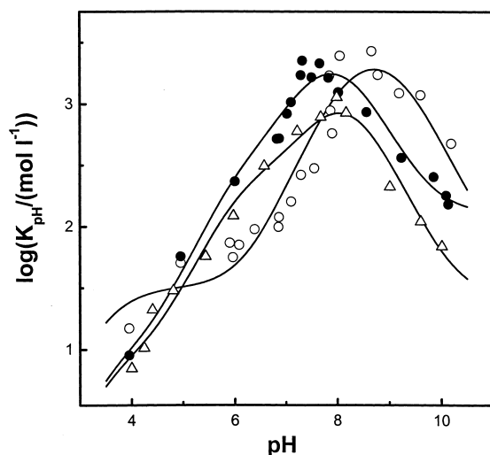
Fig. 3. Plot of \log K_{\text{pH}} vs pH for the PLP-TRP (○), PLP-MTRP (●), and PLP-BTRP (△) systems. Curves calculated using Eq. 9 and data from Table 1.
