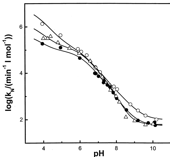
Fig. 4. Plot of \log k_N vs pH for the PLP-TRP (○), PLP-MTRP (●), and PLP-BTRP (△) systems. Curves calculated using theoretical values of k_1 .
