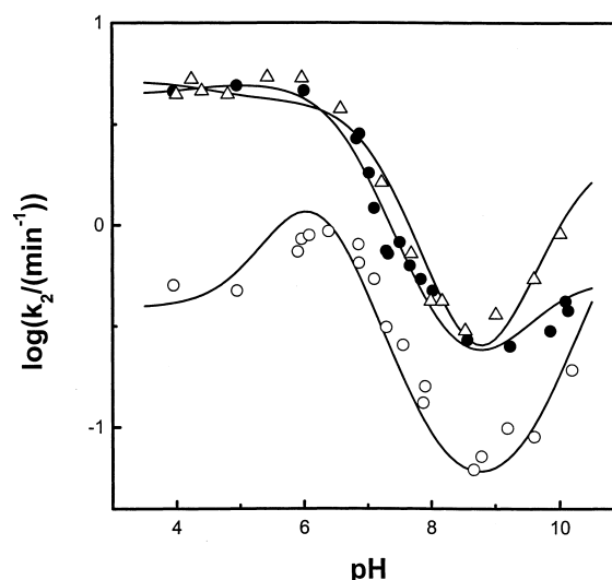
Fig. 2. Plot of \log k_2 vs pH for the PLP–TRP (○), PLP–MTRP (●), and PLP–BTRP (△) systems. Curves calculated using Eq. 8 and data from Table 1.
