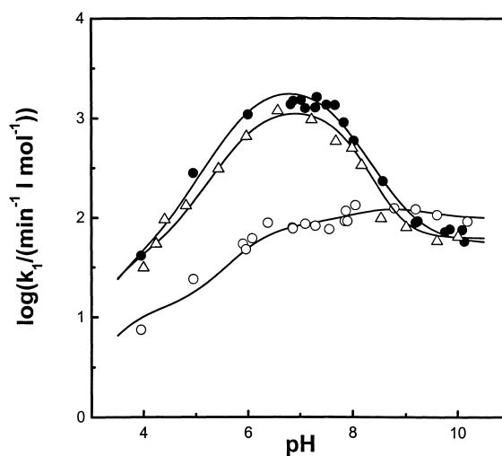
Fig. 1. Plot of \log k_1 vs pH for the PLP–TRP (○), PLP–MTRP (●), and PLP–BTRP (△) systems. Curves calculated using Eq. 7 and data from Table 1.
